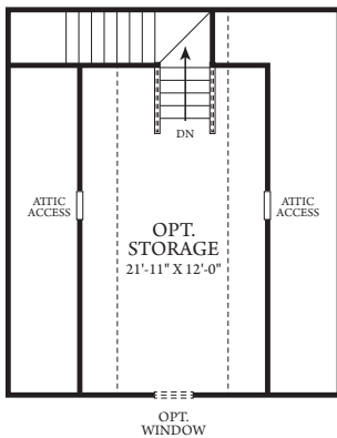
OPT. STORAGE OVER GARAGE
