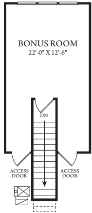
OPT. SECOND FLOOR BONUS ROOM
