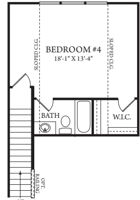
OPT. BEDROOM #4 W/ BATH
