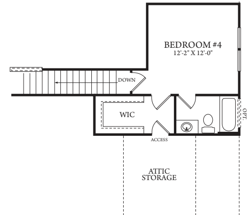
BEDROOM #4/BATH #3
